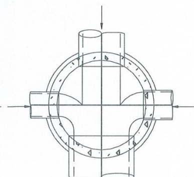
THROUGH PIPE TWO COLLECTION LINES
