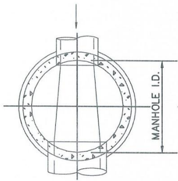
THROUGH PIPE
